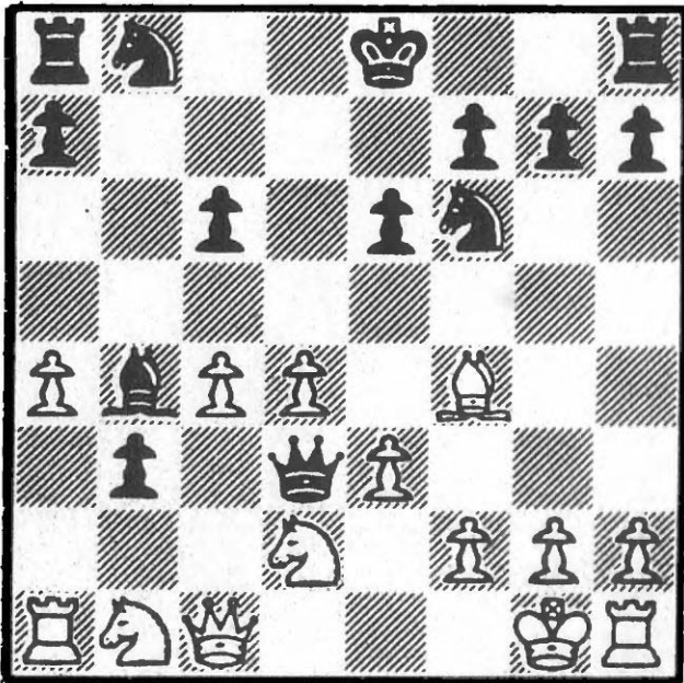
120 After 16 Ncb1
